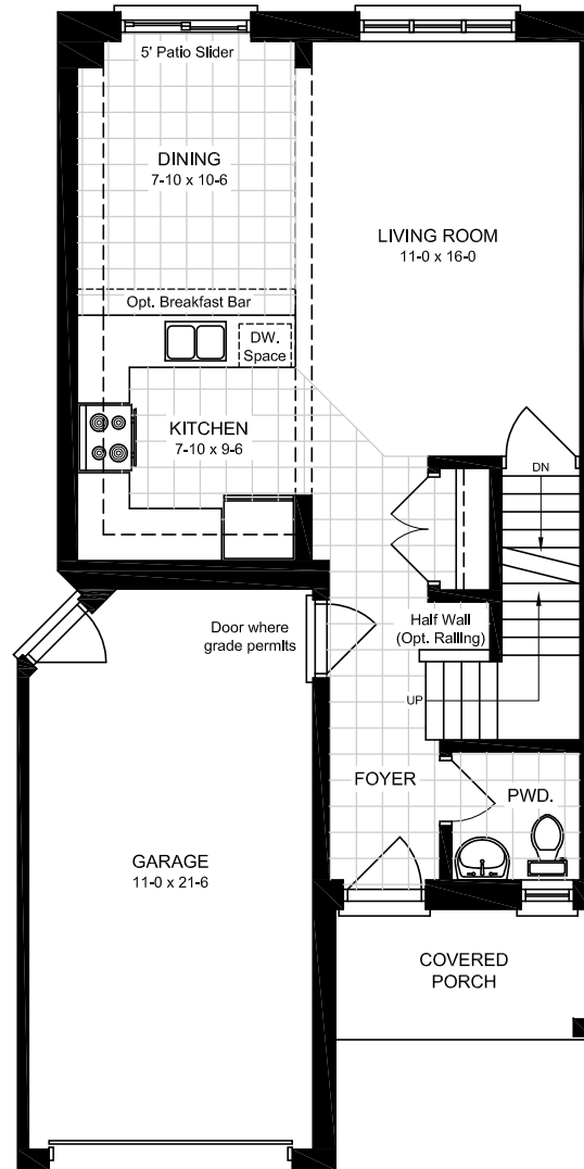
MAIN FLOOR PLAN - M2
