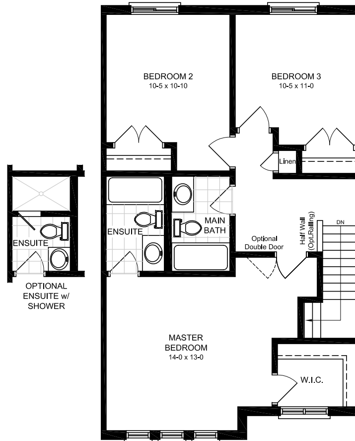
SECOND FLOOR PLAN - S2
