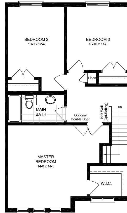
SECOND FLOOR PLAN - S1
