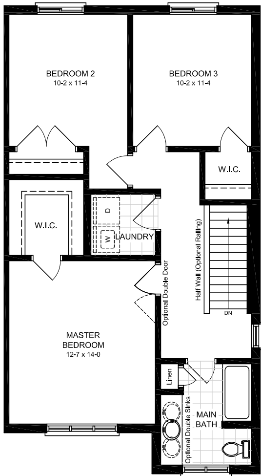
SECOND FLOOR PLAN - S2
