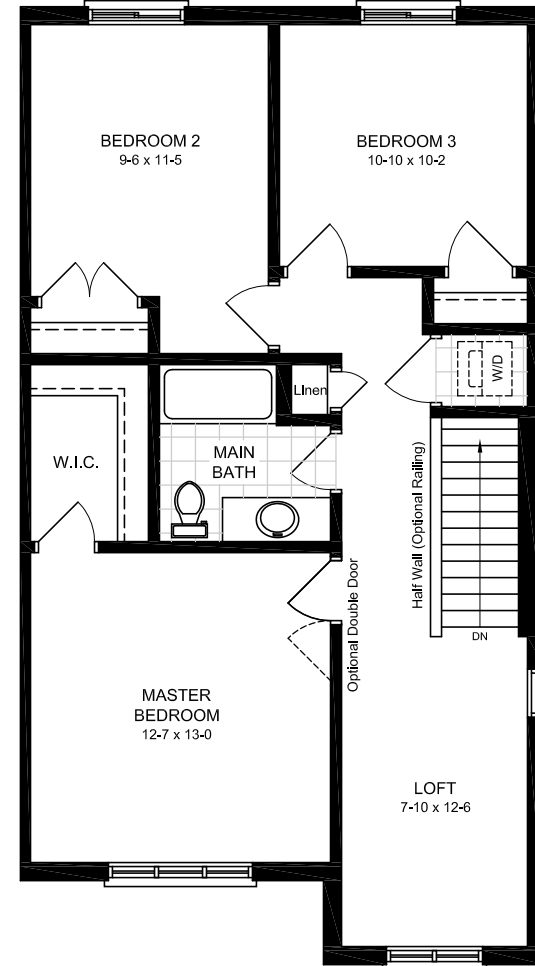
SECOND FLOOR PLAN - S1
