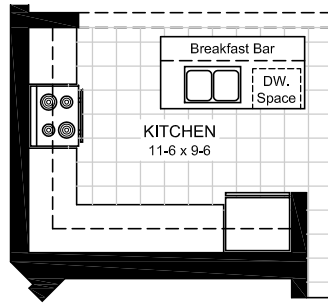
MAIN FLOOR PLAN - M2
