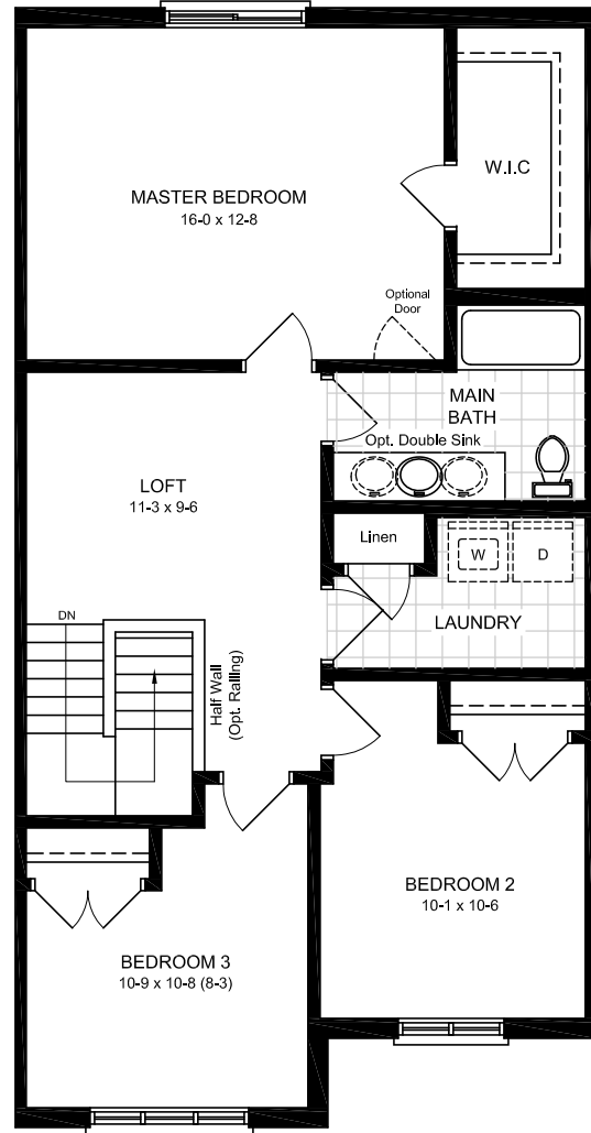
SECOND FLOOR PLAN - S1
