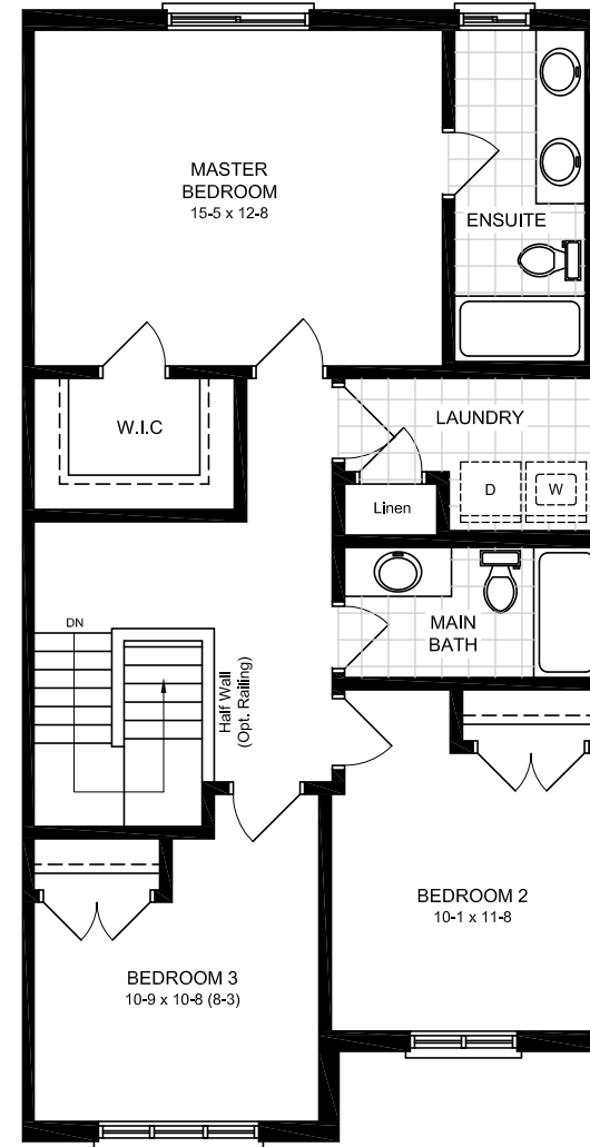
SECOND FLOOR PLAN - S3
