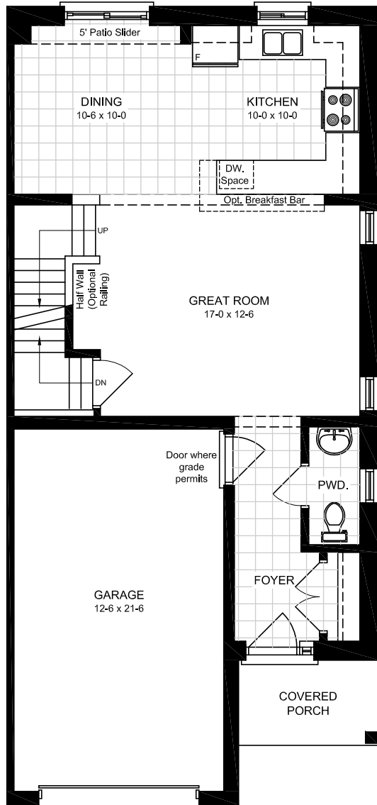
MAIN FLOOR PLAN - M1
