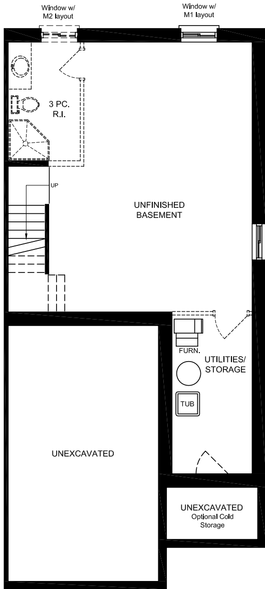
BASEMENT FLOOR PLAN
